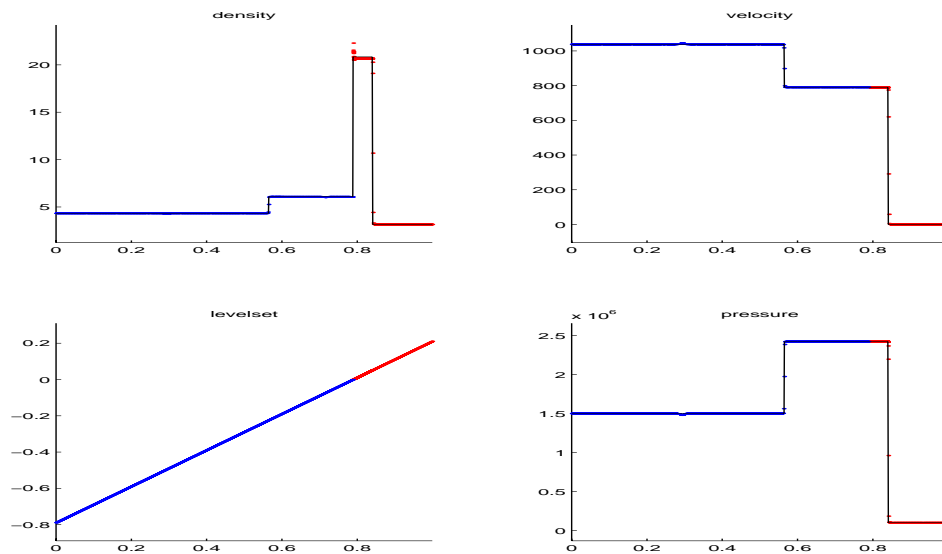
Figure 10: Test D, case 2 - after one level of grid refinement.
