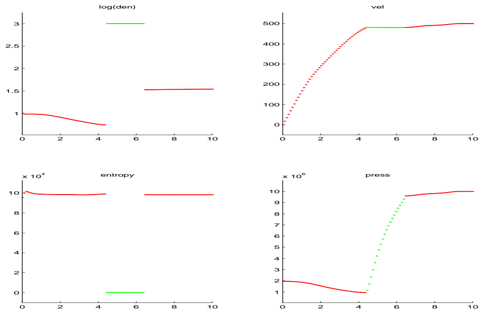
Figure 4: gamma law gas (RED) & water (GREEN), 100 grid cells.
