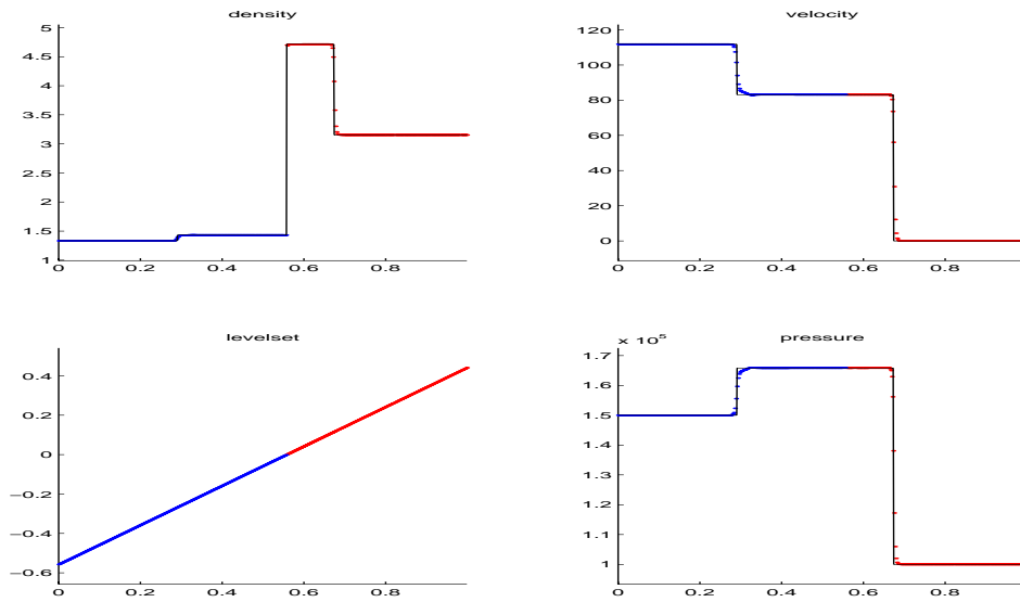
Figure 8: Test C - similar to test B, except a different material is used on the Lagrangian grid to the right of the interface. The initial shock wave is again moving from left to right.
