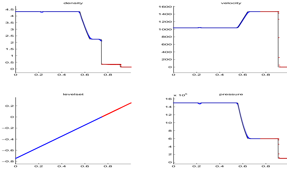
Figure 7: Test D, case 1 - similar to test B, except a stronger shock wave propagates from the Eulerian grid (left) towards the Lagrangian grid (right) impinging upon the interface.
