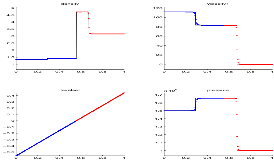
Figure 14: Test C in two spatial dimensions - side view.
