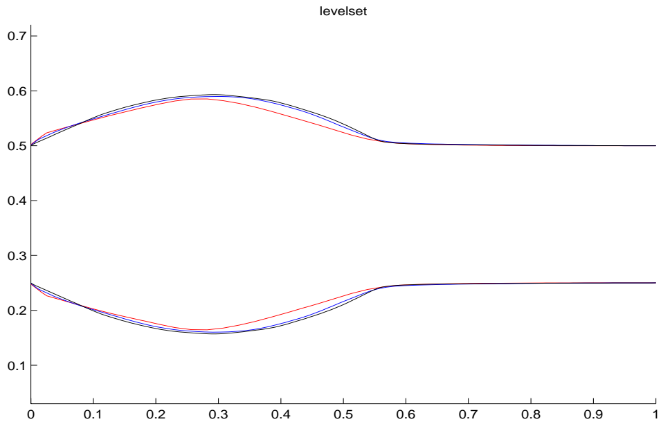
Figure 16: Interface location at t = .0004 seconds for 3 different grids.
