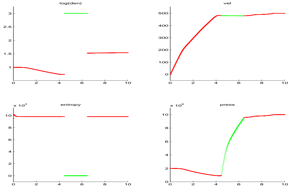
Figure 3: gamma law gas (RED) & water (GREEN), 400 grid cells.
