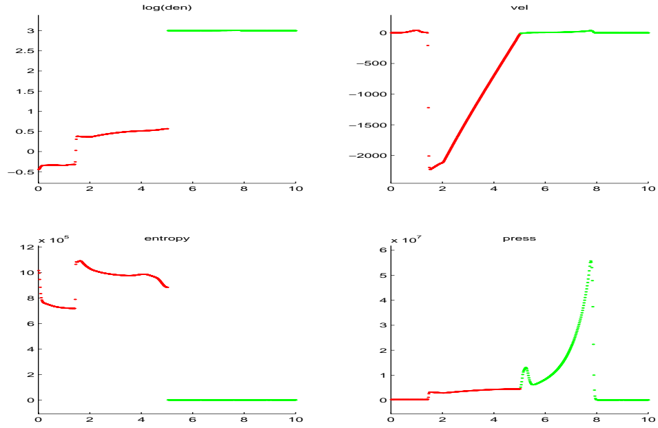
Figure 1: gamma law gas (RED) & water (GREEN), 500 grid cells.
