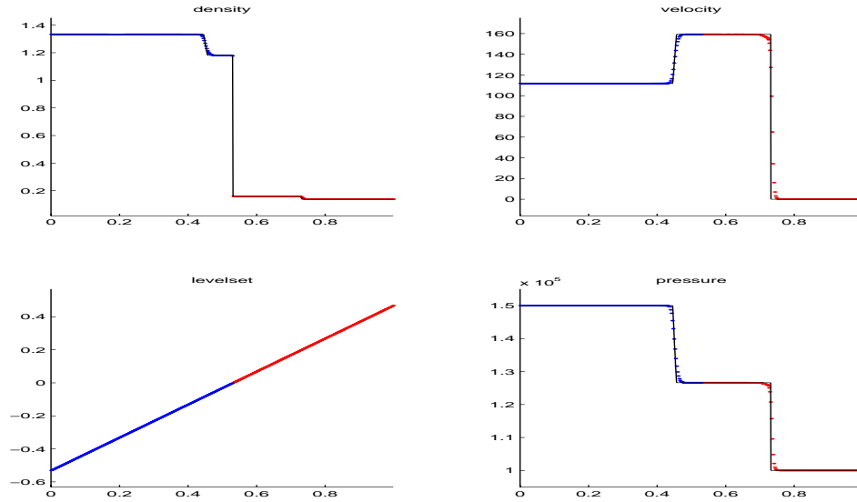
Figure 5: Test B - a shock wave propagates from the Eulerian grid (left) towards the Lagrangian grid (right) producing both reflected and transmitted waves when it hits the multimaterial interface in between the grids.
