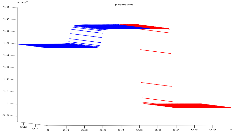
Figure 13: Test C in two spatial dimensions - a shock wave propagates from the Eulerian grid (left) towards the Lagrangian grid (right) producing both reflected and transmitted waves when it hits the multimaterial interface in between the grids.
