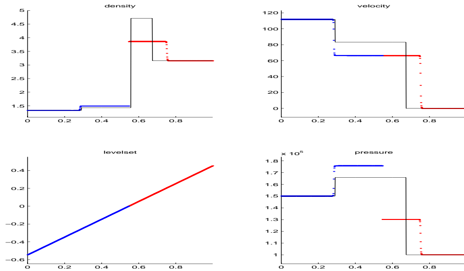
Figure 12: Test C with material strength in the Lagrangian fluid (right) after one level of grid refinement.
