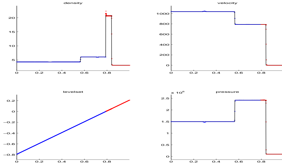
Figure 9: Test D, case 2 - similar to test C, except a stronger shock wave propagates from the Eulerian grid (left) towards the Lagrangian grid (right) impinging upon the interface.
