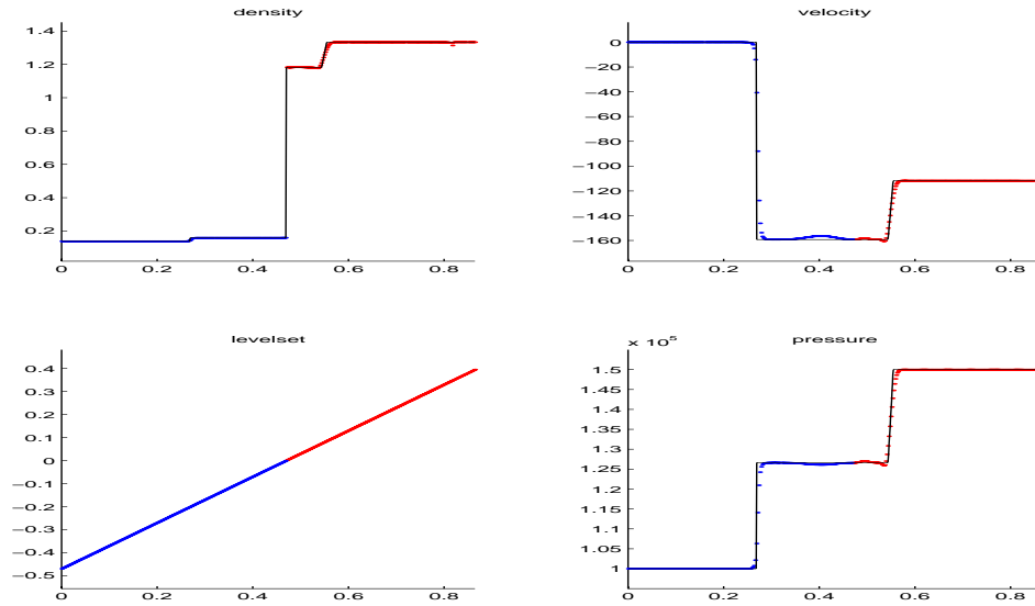
Figure 6: Test B - a shock wave propagates from the Lagrangian grid (right) towards the Eulerian grid (left) producing both reflected and transmitted waves when it hits the multimaterial interface.
