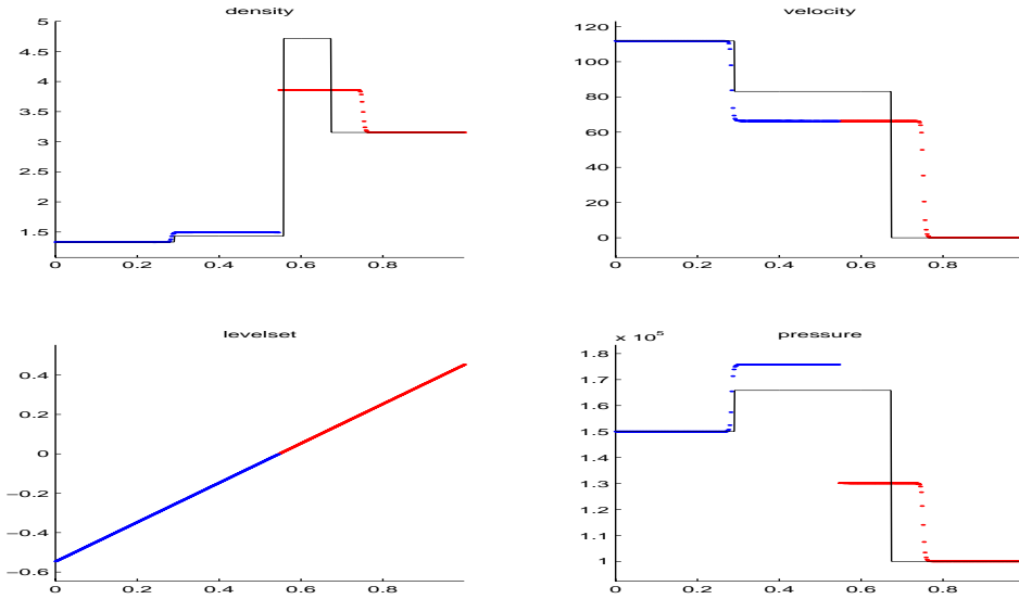
Figure 11: Test C with material strength in the Lagrangian fluid (right). The material strength is balanced at the interface by the jump in pressure producing a continuous normal stress. The solid line shows the exact solution to this problem without material strength.
