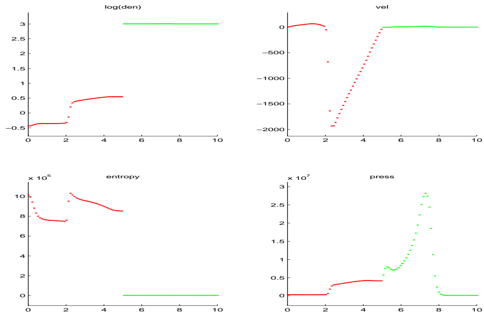
Figure 2: gamma law gas (RED) & water (GREEN), 100 grid cells.
