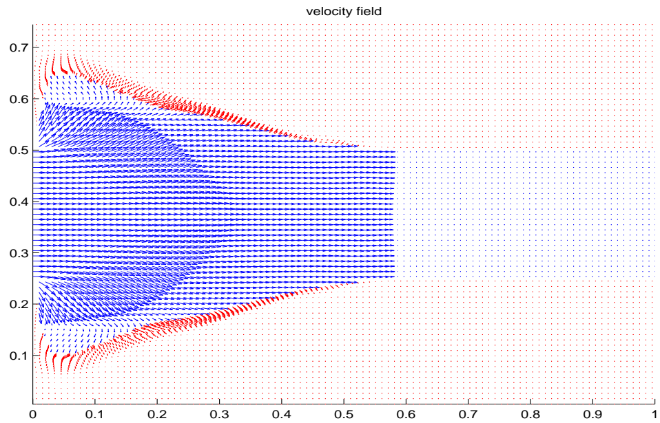
Figure 20: Velocity field at t = .0004 seconds.
