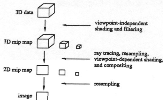
Figure 4: Rendering pipeline
