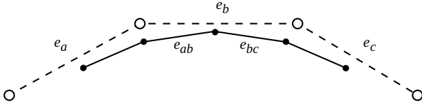
Figure 13: Subedge labeling.
