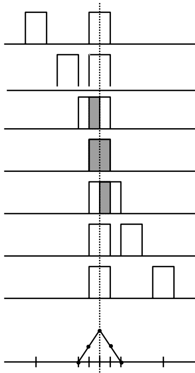
Figure 10: Convolution of two square pulses
