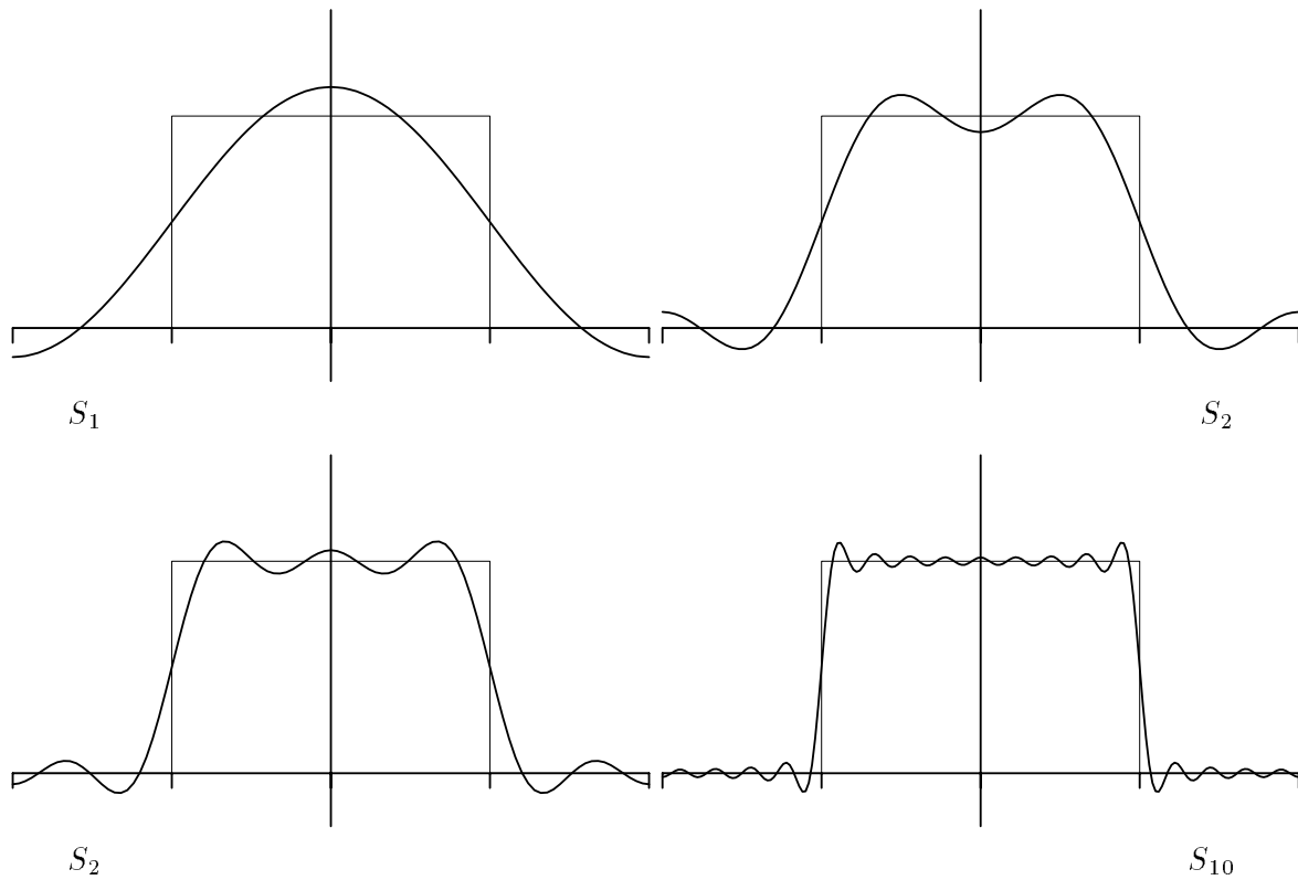
Figure 4: Four approximations to a square pulse. Notice that each approximation involves higher frequency terms and the resulting sum more closely approximates the pulse. As more and more high frequencies are added, the sum converges exactly to the square pulse. Note also the oscillation at the edge of the pulse; this is often referred to as the Gibbs phenomenon, or ringing.
