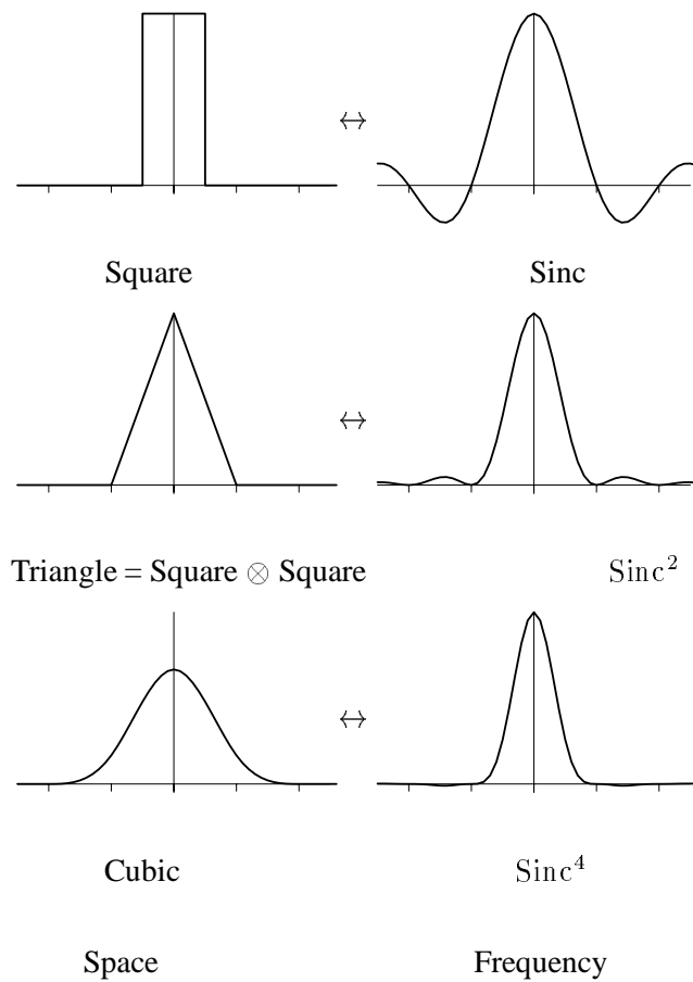
Figure 11: The results of convolving a square pulse with itself multiple times.
