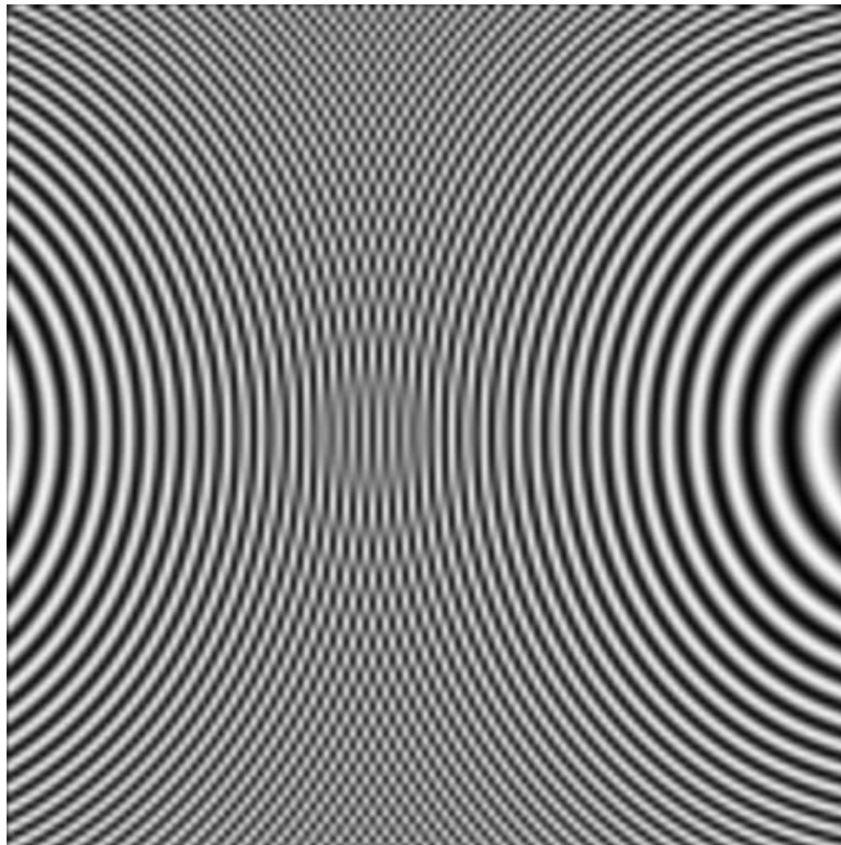
Figure 3: Sampling the equation \sin(x^2 + y^2) . Rather than a single set of rings centered at the origin, notice there are several sets of superimposed rings beating against each other to form a pronounced Moire pattern.
