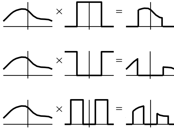
Figure 7: Perfect low-pass (top), high-pass (middle), and band-pass (bottom) filters.
