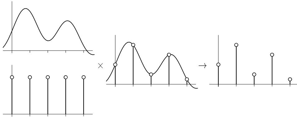
Sampling in the Space Domain
