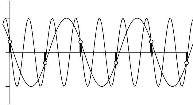
Figure 15: Sampling a sine wave. Sampling the function \sin 1.5\omega x yields the same values as sampling the function \sin 0.5\omega x . Thus, the higher frequency 1.5\omega which is above the Nyquist frequency, cannot be distinguished from the lower frequency 0.5\omega .
