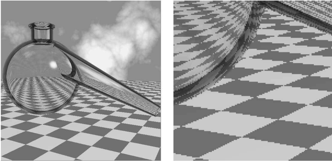
Figure 2: A ray traced image of a 3D scene. The image is shown at full resolution on the left and magnified on the right. Note the jagged edges along the edges of the checkered pattern.
