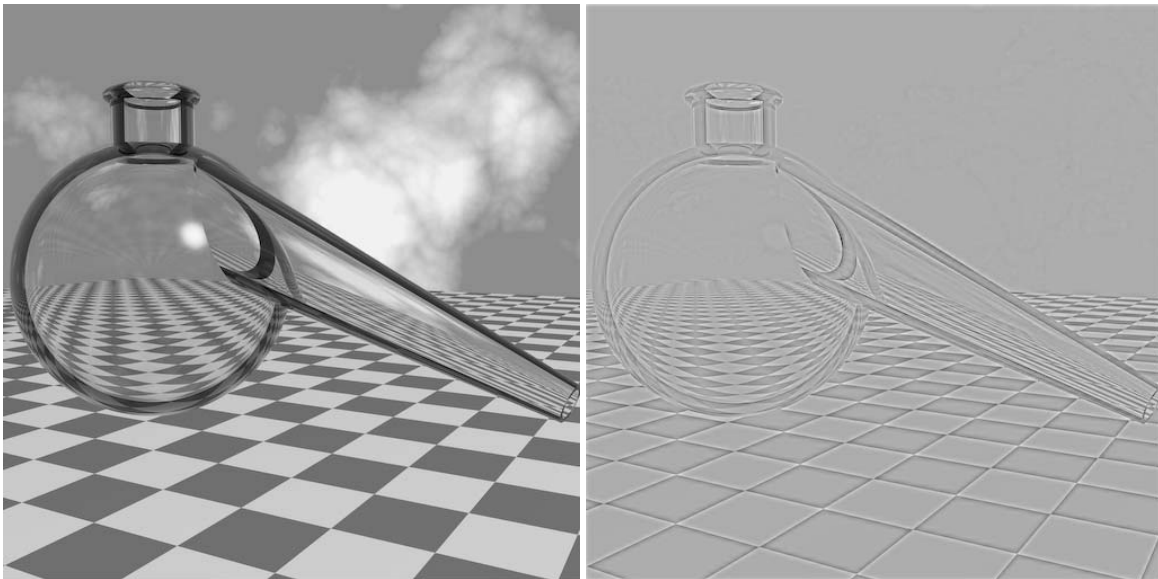
Figure 9: Application of a high-pass filter to an image. Notice that in the resulting image the low frequencies have been removed and only places in the image that are changing, such as edges, remain.
